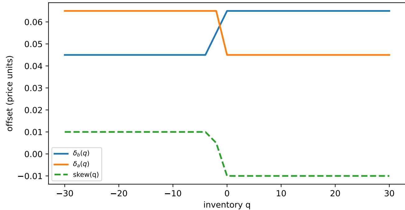
HJB policy slice (fixed t , S , \lambda_{\pm} )
