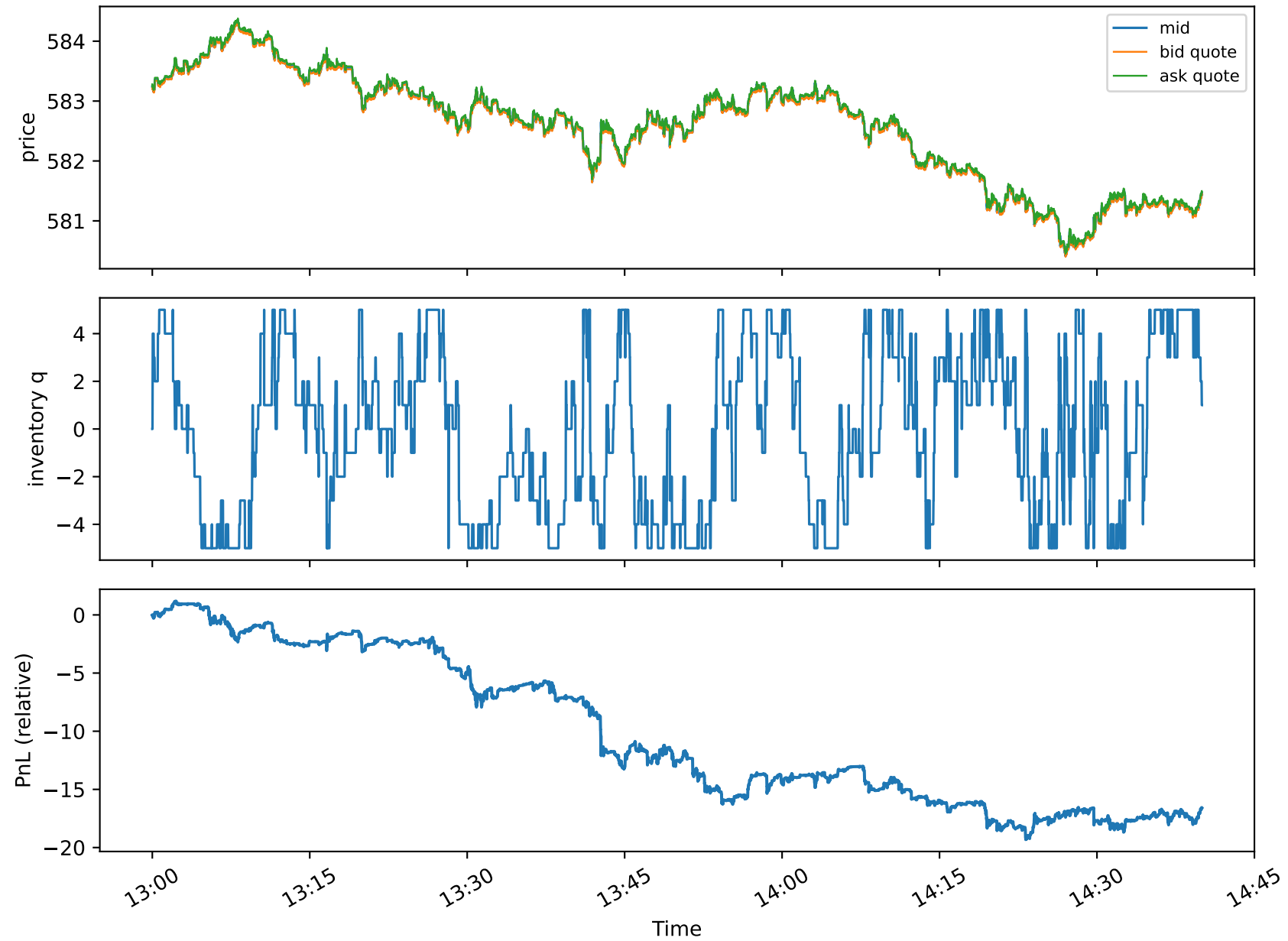
Backtest path: quotes, inventory, PnL
