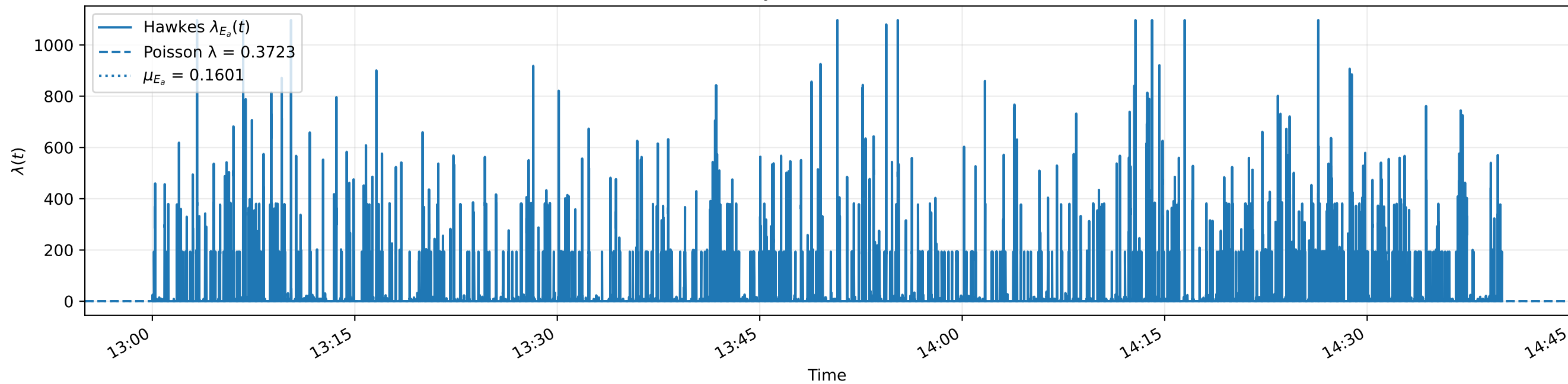
Intensity: Hawkes vs Poisson
