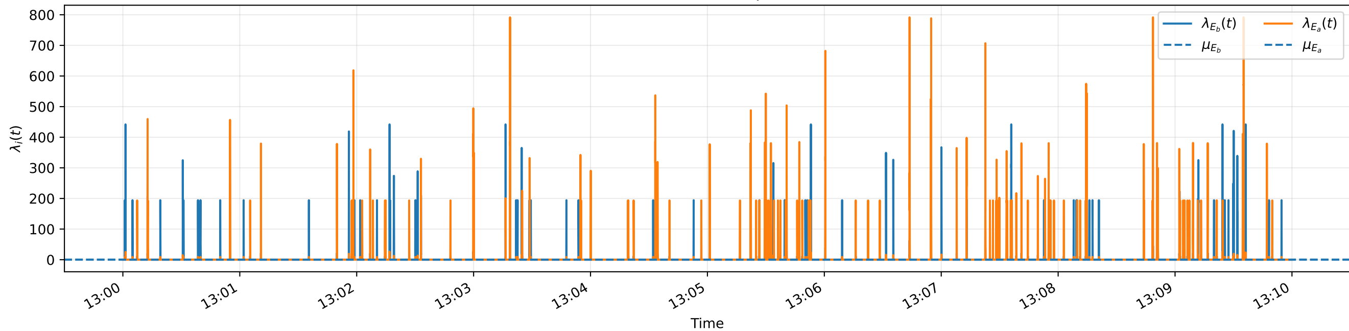
Intensities of the two processes
