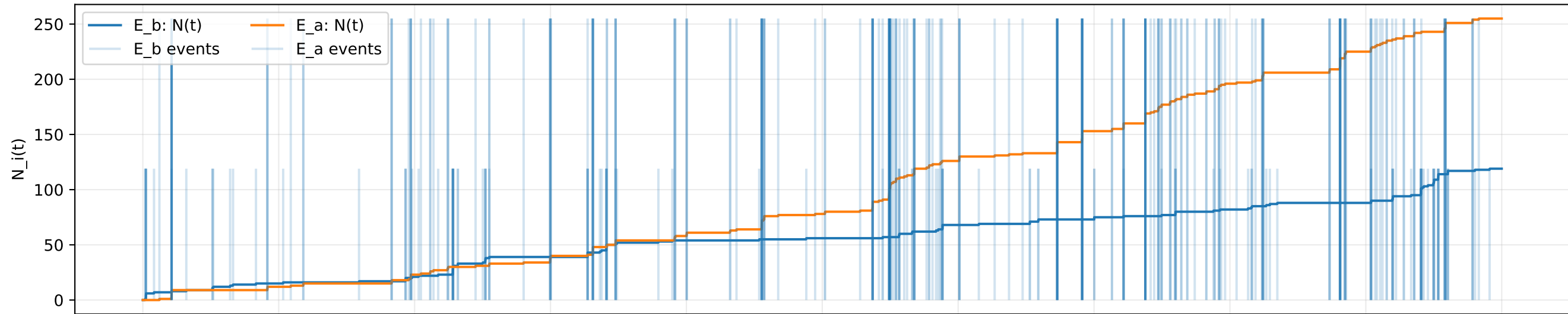
Hawkes 2D — Counting processes + event times
