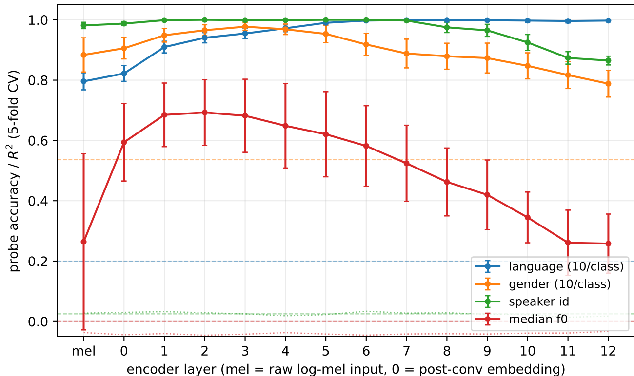
Property decodability across whisper-small encoder layers
