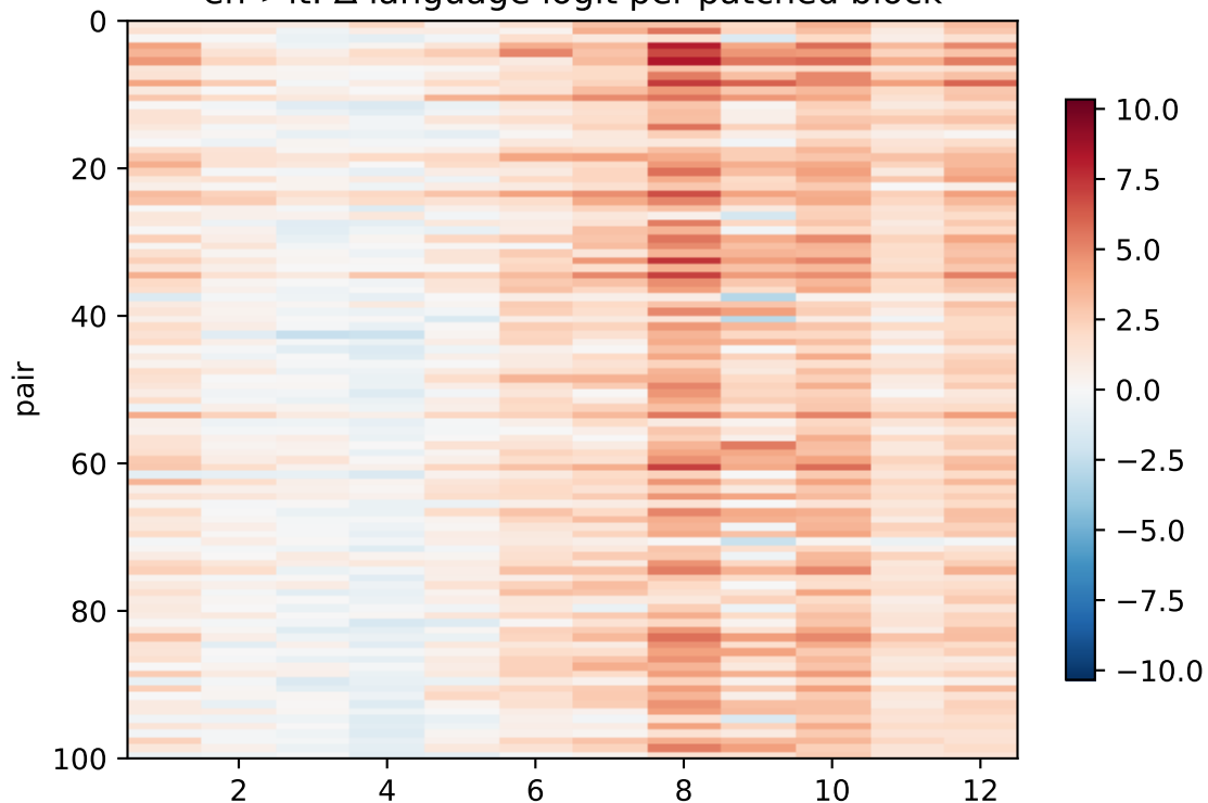
en->it: \Delta language logit per patched block
