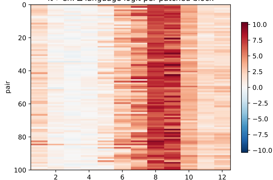
it->en: \Delta language logit per patched block
