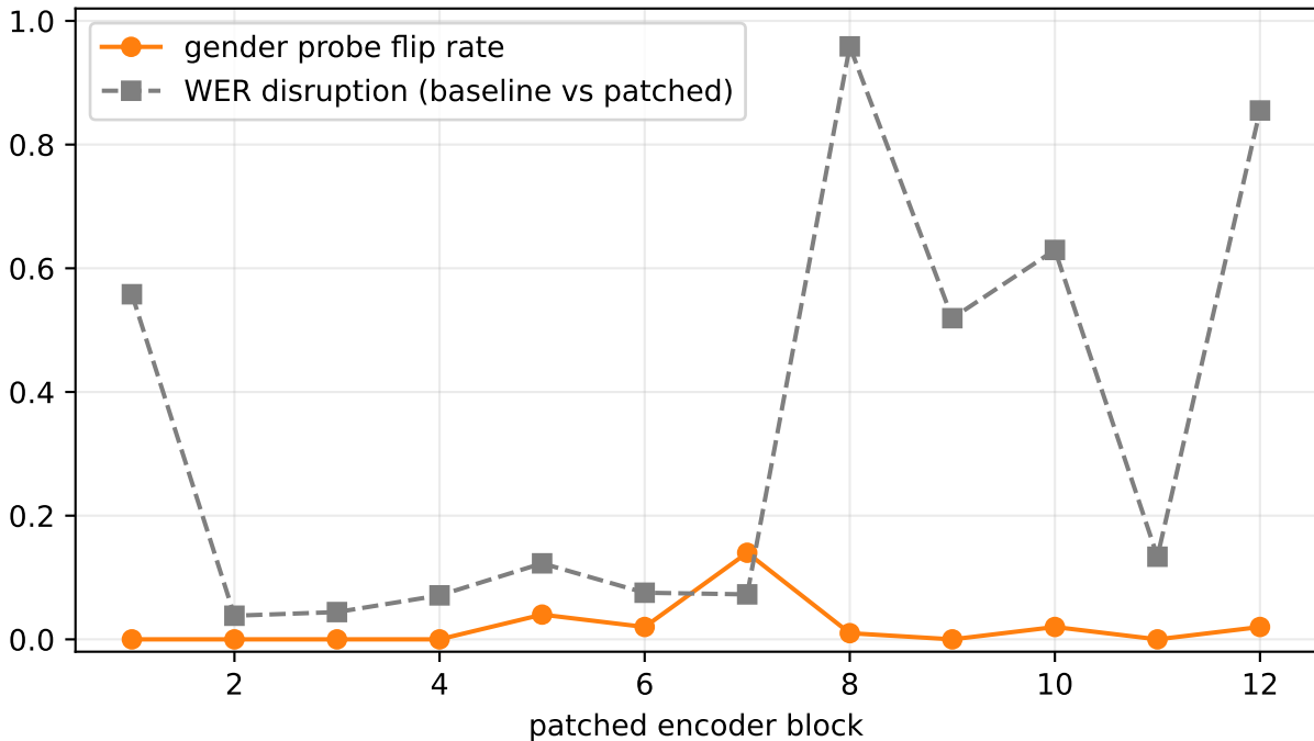
Gender block-update patching, openai/whisper-small
