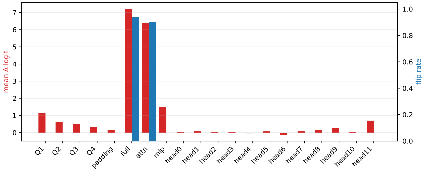
Partial patches of block 8 (it->en), openai/whisper-small
