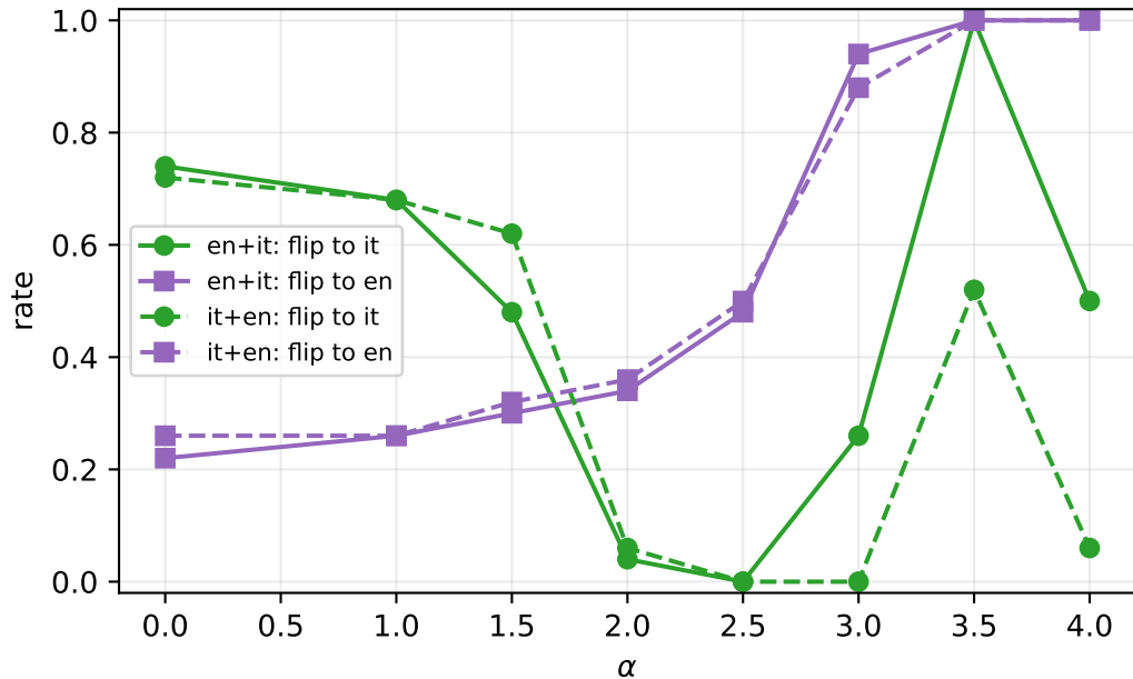
code-switched clips
