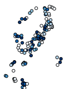
chr10_128568737_C_T A (C=0.13*)
