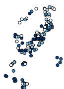
chr14_95974143_C_T I (C=0.12*)
