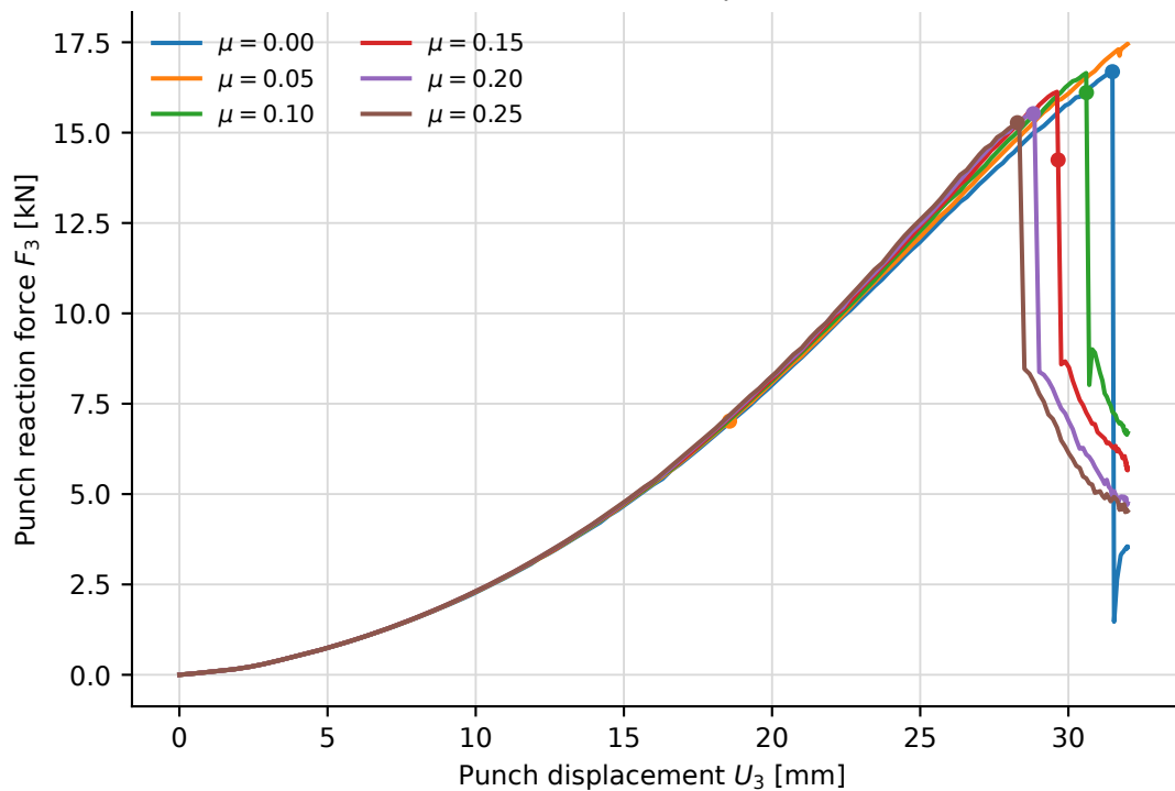
Punch force response
