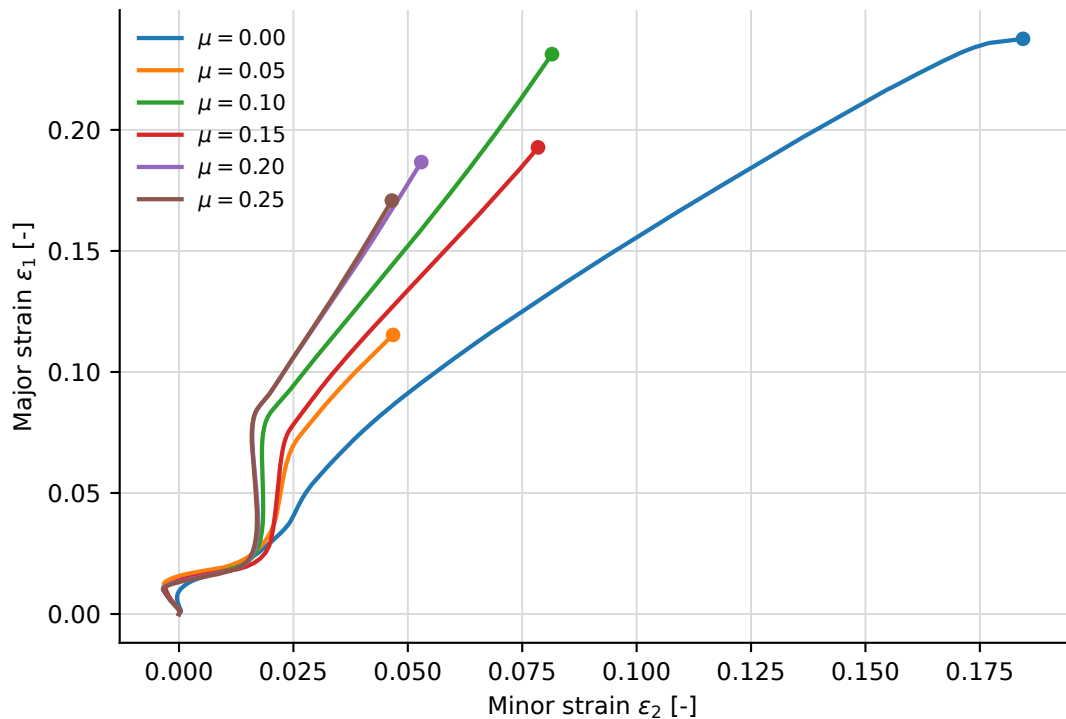
Punch/blank friction sensitivity (W120)
