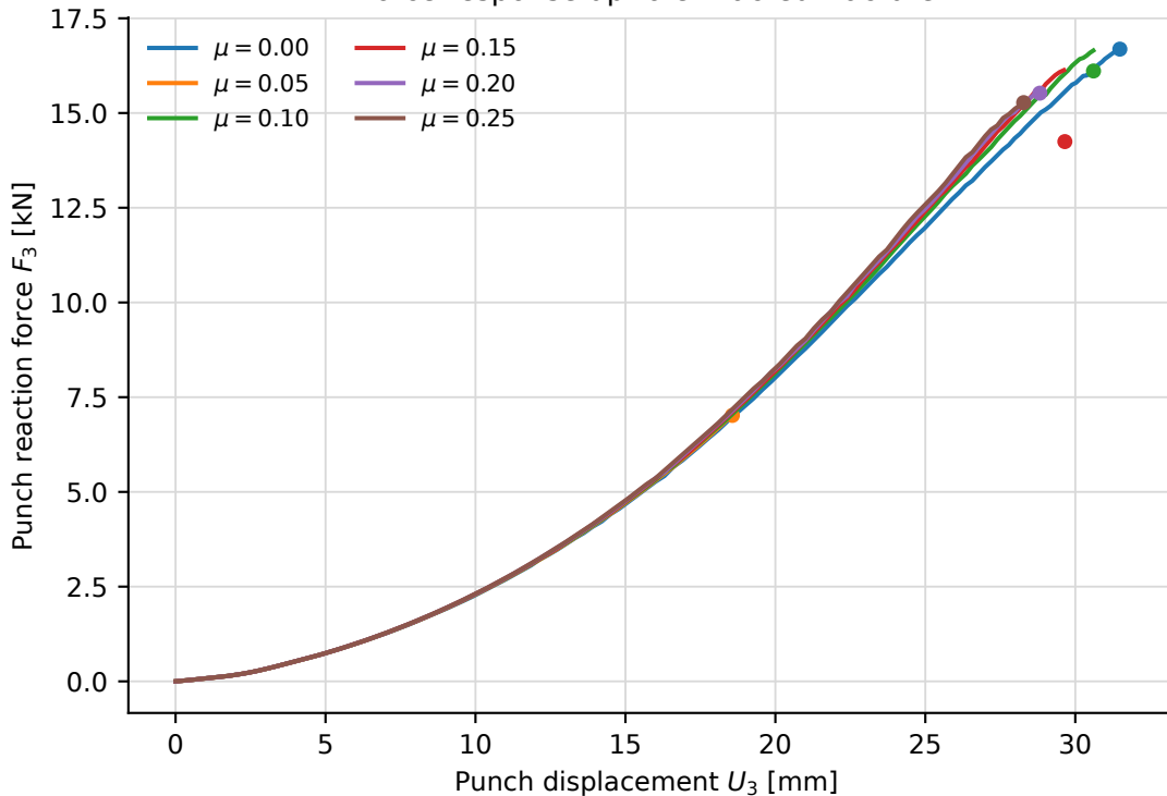
Force response up to extracted fracture
