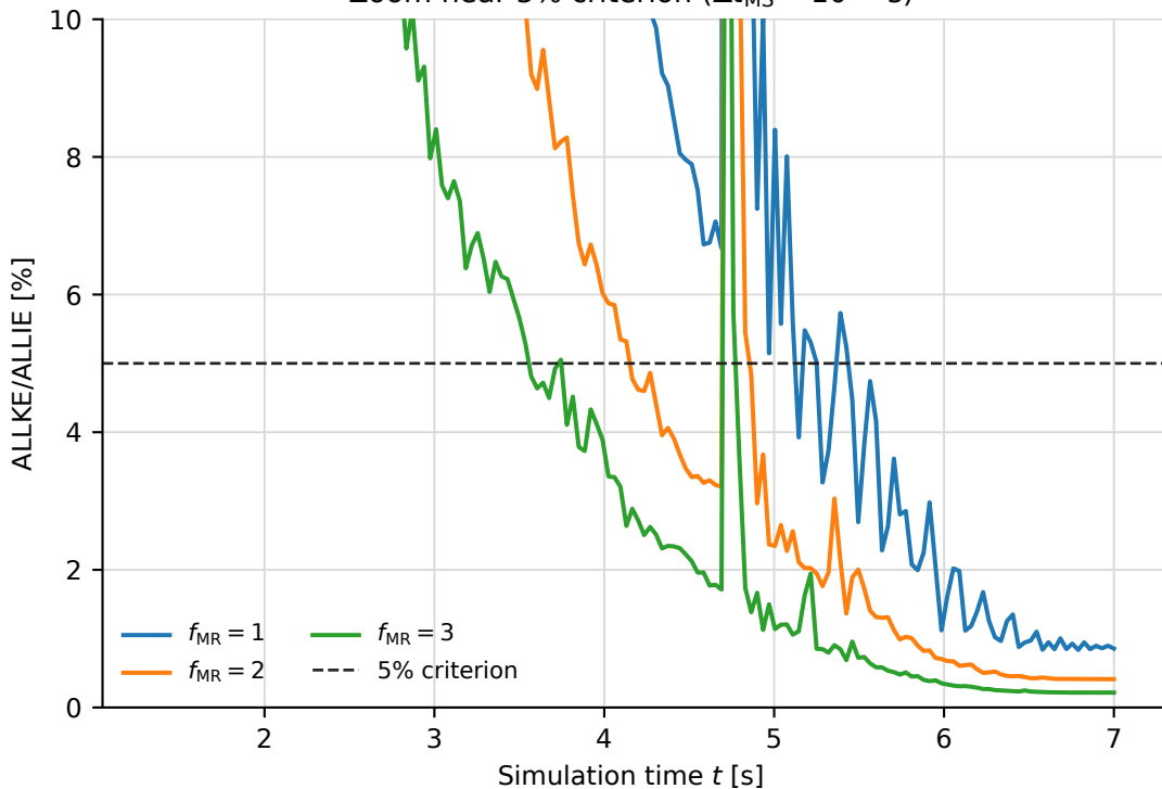
Zoom near 5% criterion ( \Delta t_{\text{MS}} = 10^{-5} s)
