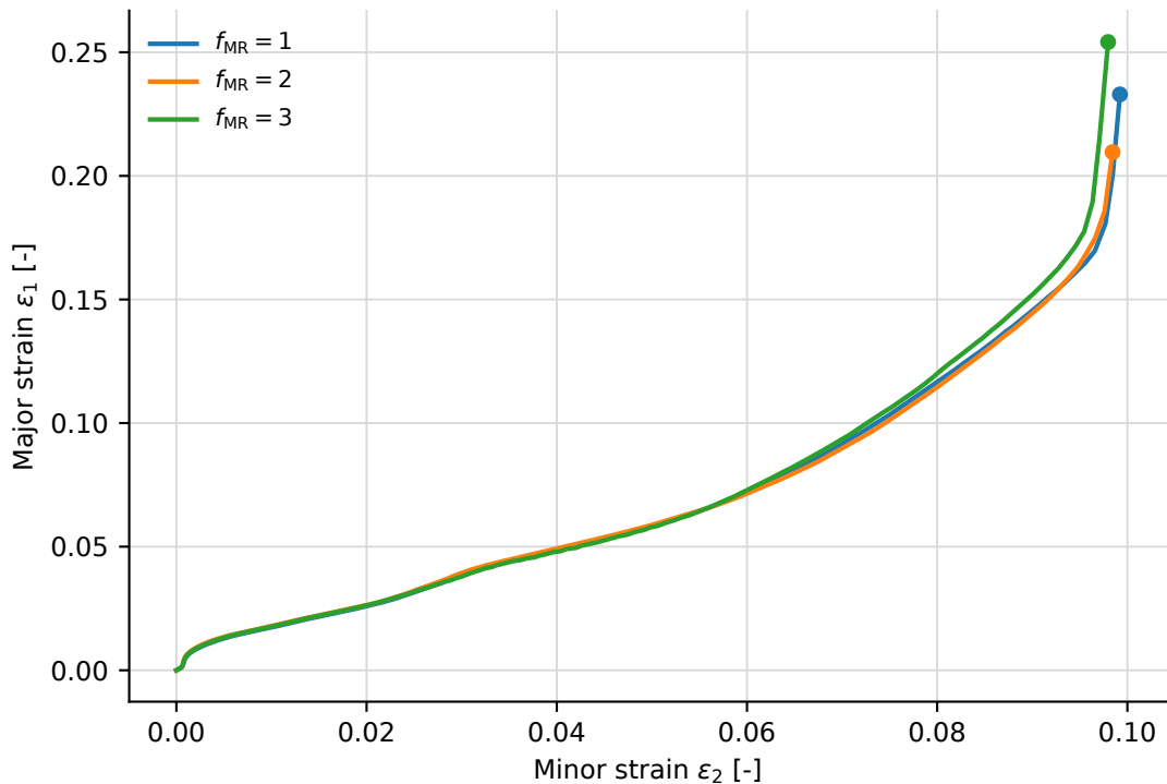
Mesh-refinement sensitivity ( \Delta t_{\text{MS}} = 10^{-5} s)
