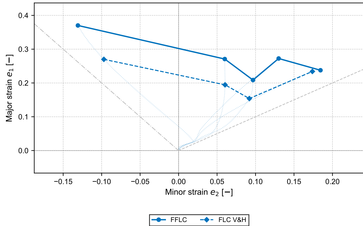
FLD - Nakazima > P100, P100 > ms1e6
