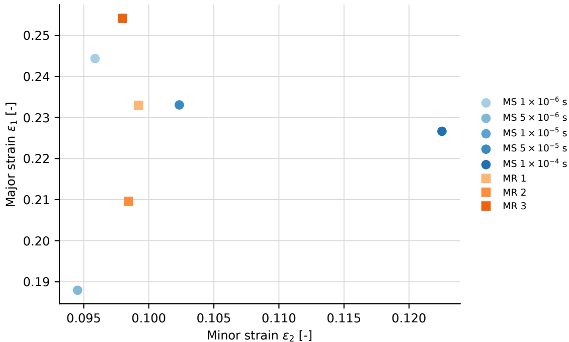
Extracted fracture forming-limit points
