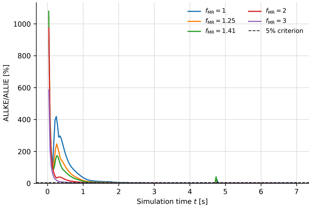
Energy-ratio history ( \Delta t_{\text{MS}} = 10^{-6} s)
