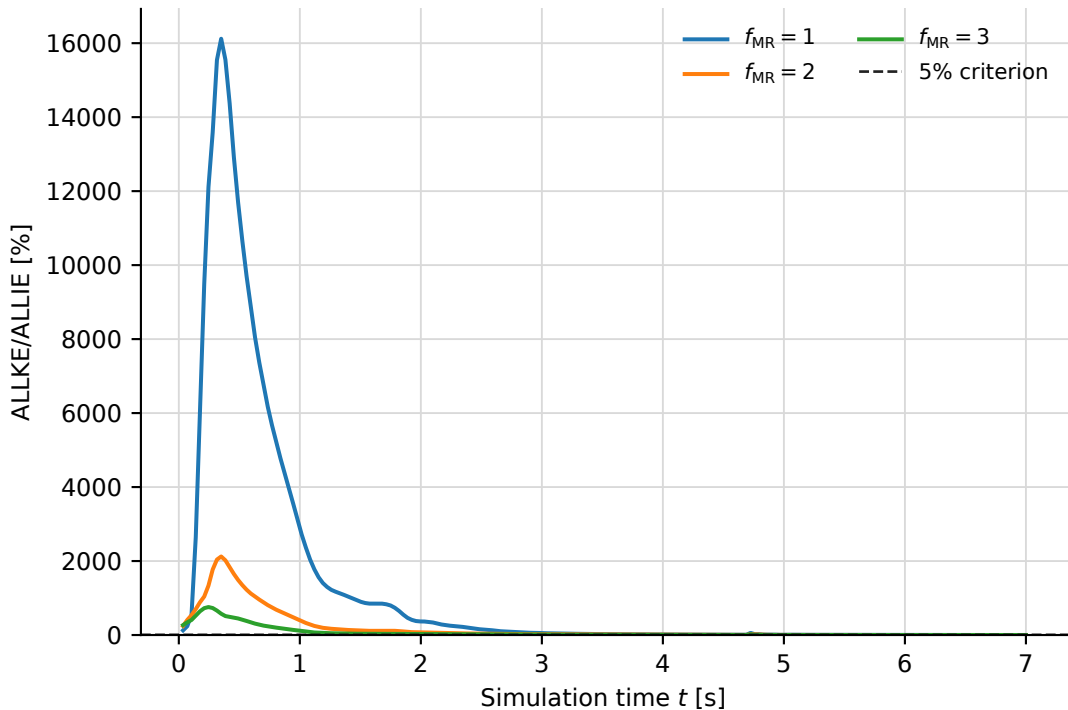
Energy-ratio history ( \Delta t_{\text{MS}} = 10^{-5} s)
