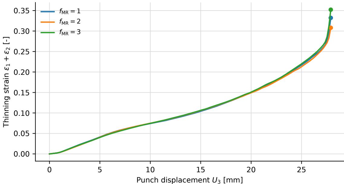
Mesh-refinement sensitivity ( \Delta t_{\text{MS}} = 10^{-5} s)
