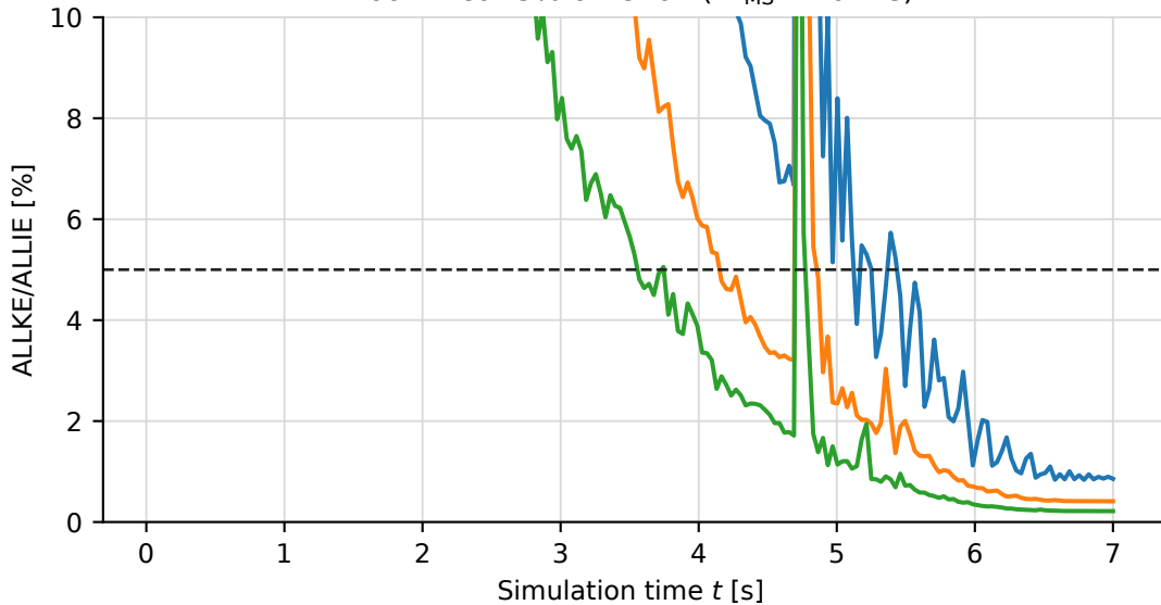
Zoom near 5% criterion ( \Delta t_{\text{MS}} = 10^{-5} s)
