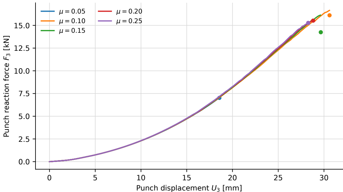
Force response up to extracted fracture
