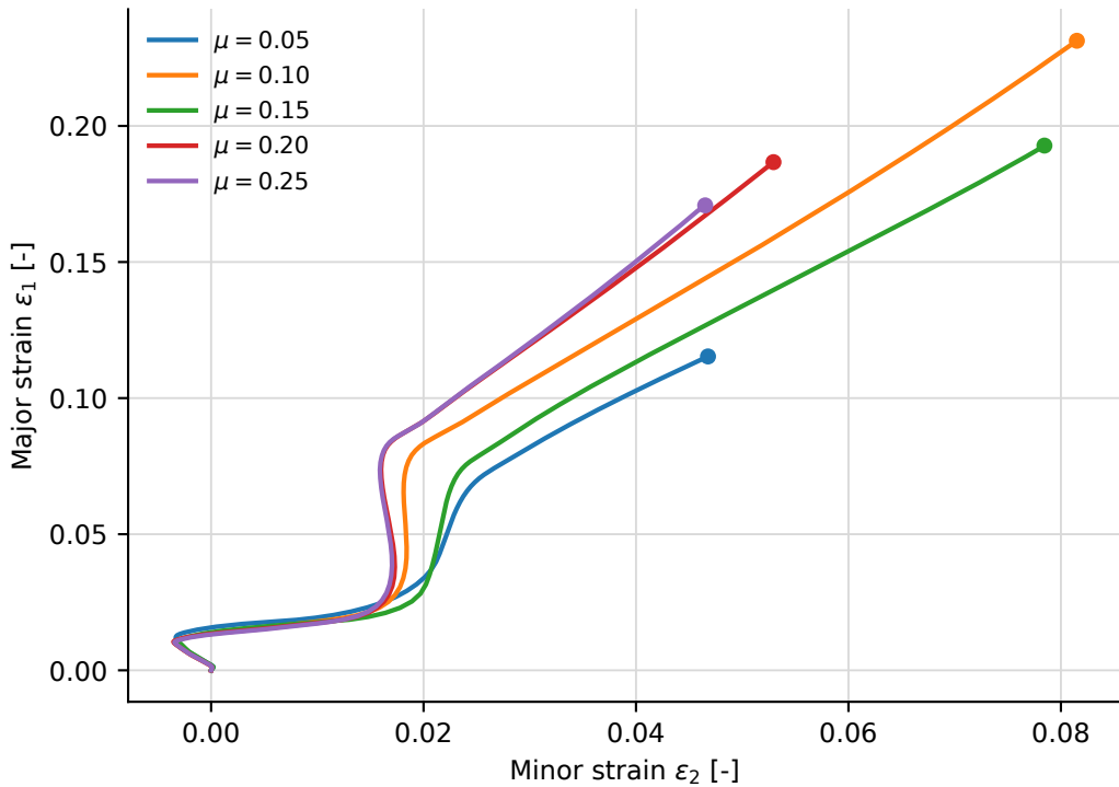
Punch/blank friction sensitivity (W120)
