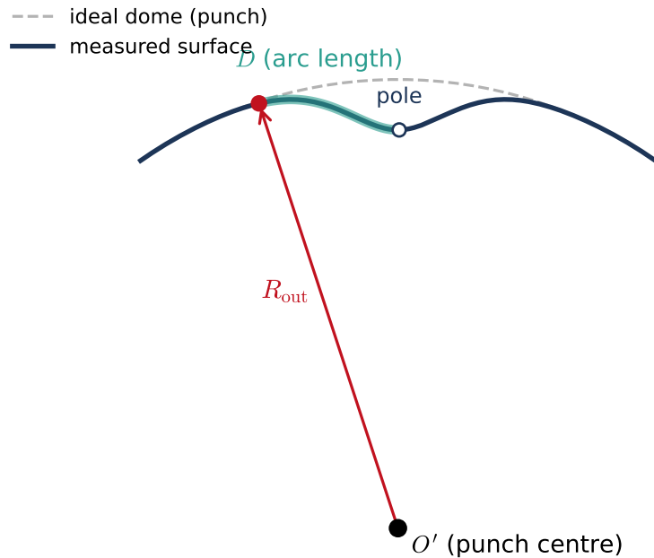
(b) Nakazima coordinates D and R_{\text{out}}
