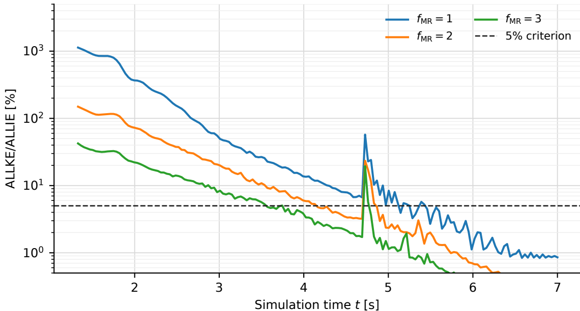
Quasi-staticity check ( \Delta t_{\text{MS}} = 10^{-5} s)
