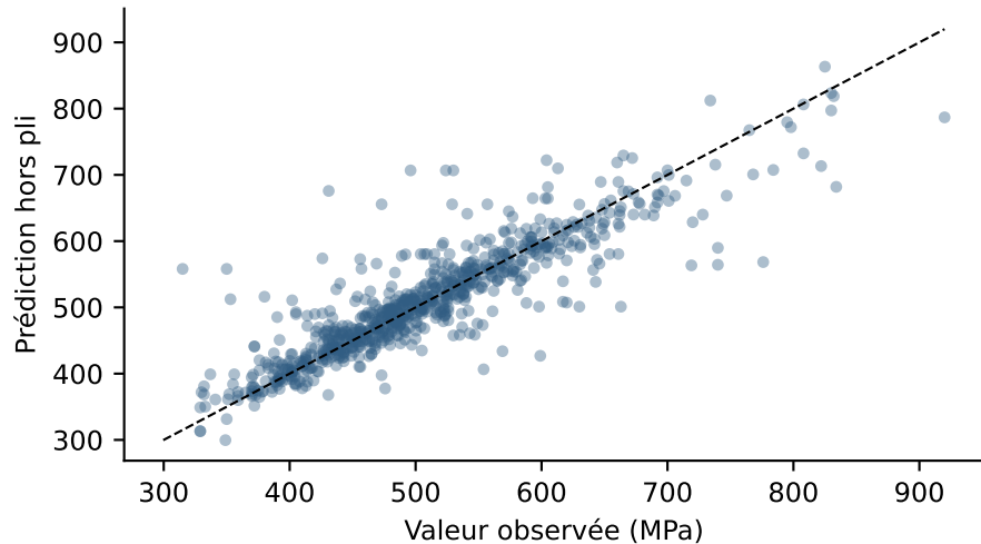
yield_strength — SVR RBF
