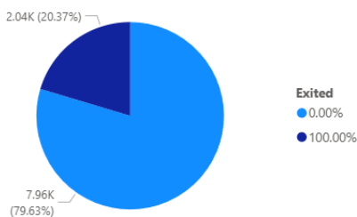
Count of CustomerId by Exited
