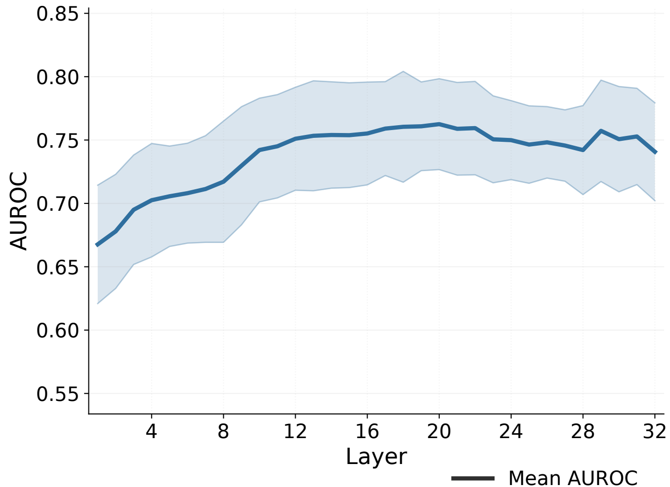
Same-language probe
