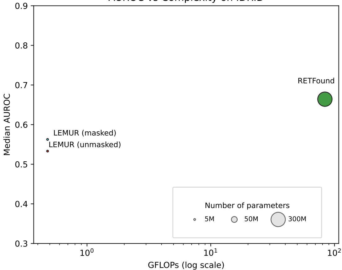
AUROC vs Complexity on IDRID
