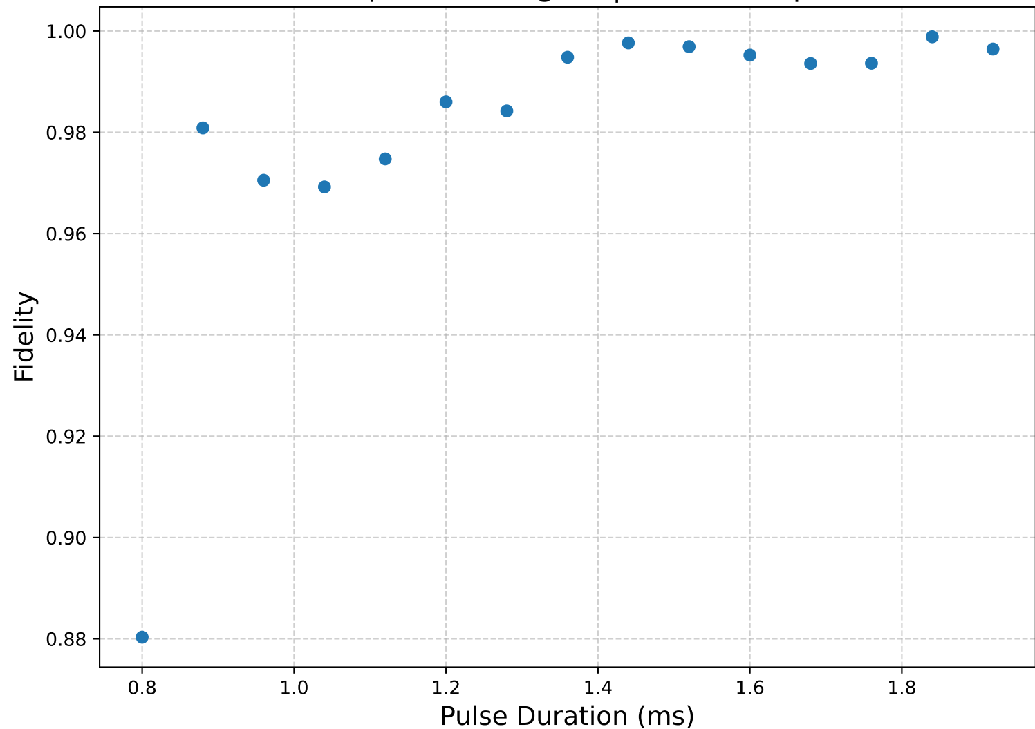
GRAPE 2 qubit CNOT gate | L-BFGS-B optimizer
