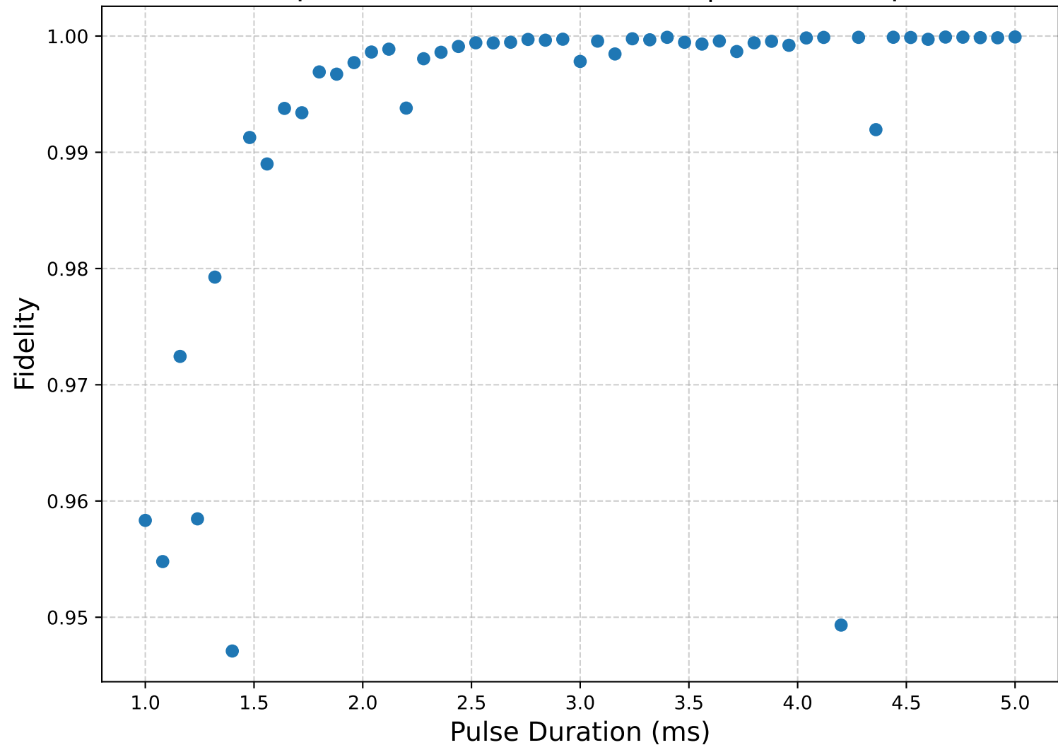
GRAPE 2 qubit destructive SWAPtest | L-BFGS-B optimizer
