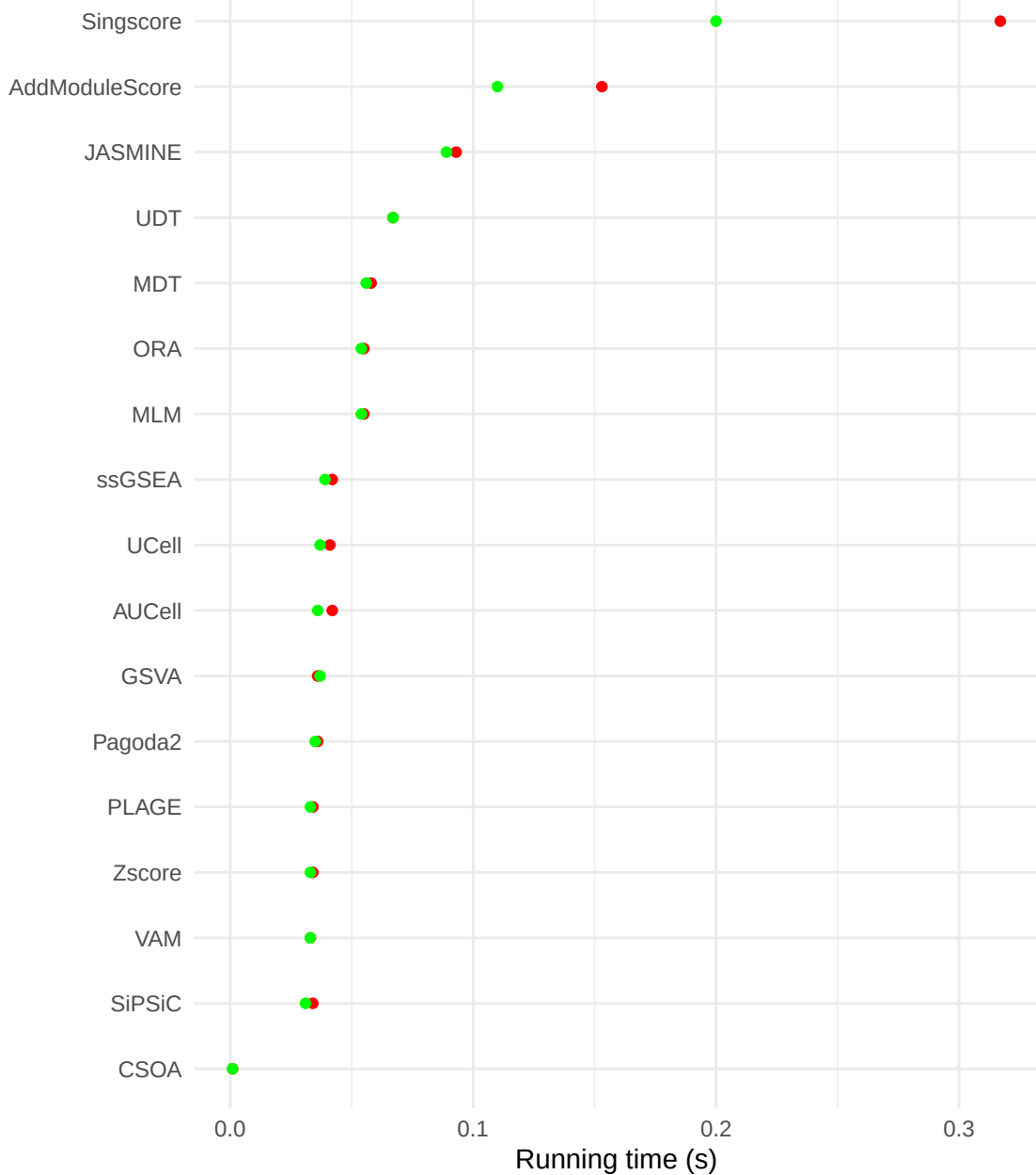
Running times
