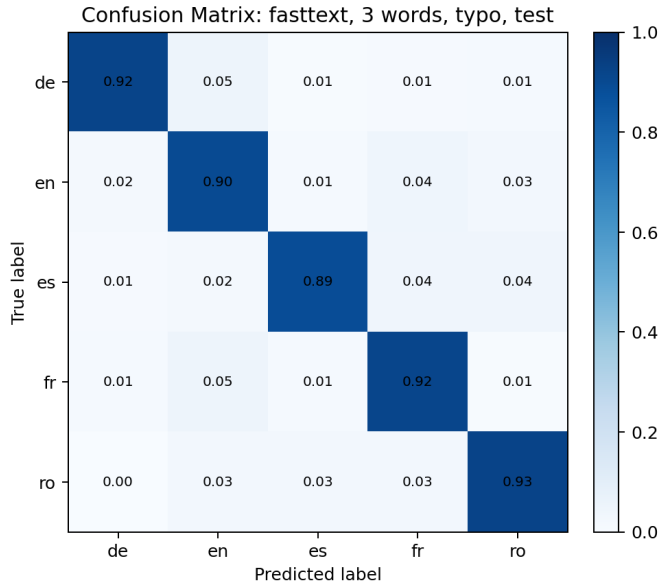
Fig. 3. Normalized confusion matrix for fastText on the hardest condition: 3-word texts with one typo on the test split.
