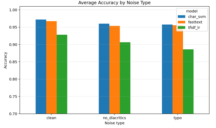
Fig. 2. Average accuracy by noise condition across models.
