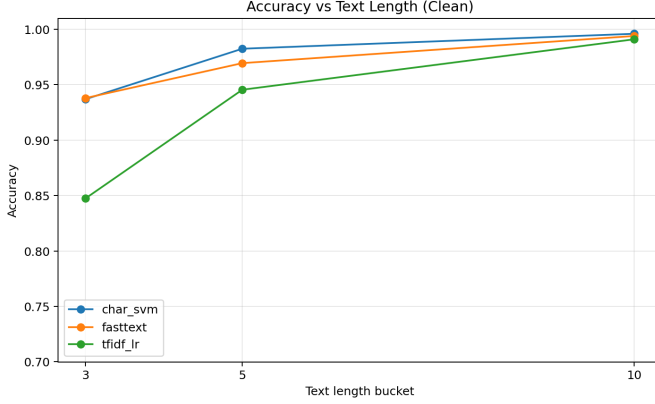
Fig. 1. Average accuracy on clean text as a function of text length.
