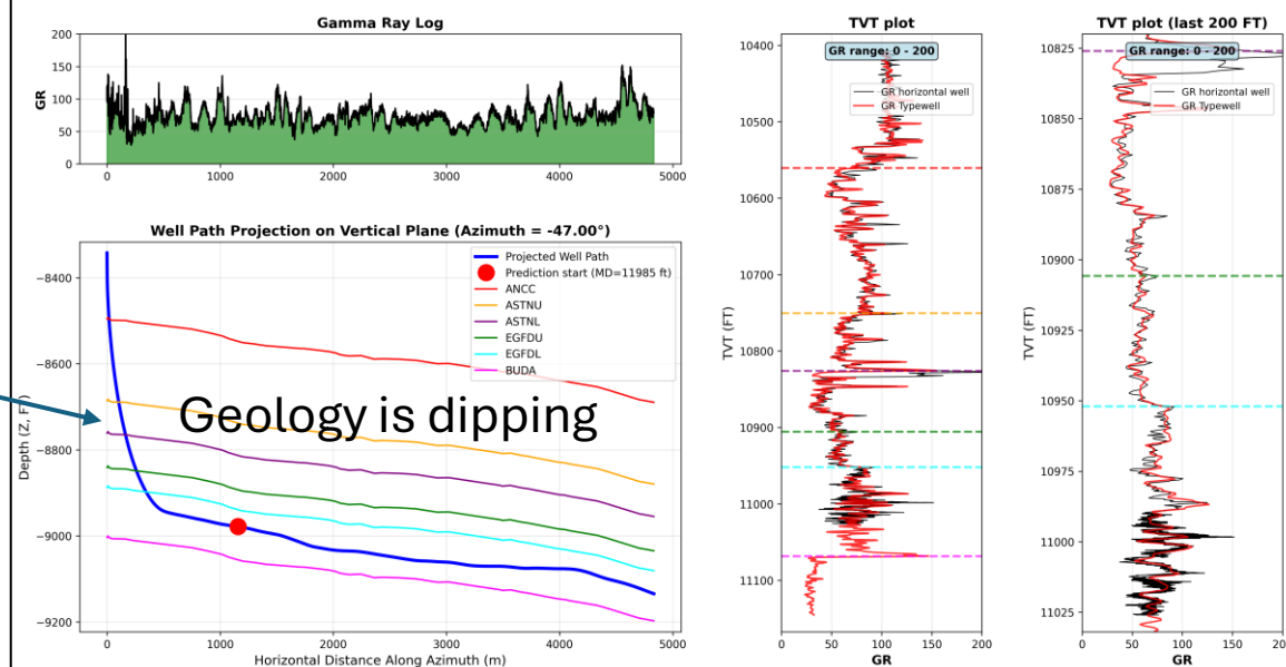
Well: Well10740 | Typewell: Typewell20003 | Azimuth = -47.00°
