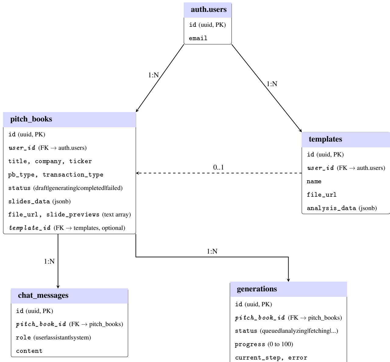
Figure 5: Database entity-relationship diagram. Primary keys in bold, foreign keys in italics. All tables use UUID primary keys with row-level security. The dashed line indicates an optional foreign key (pitch books may or may not reference a template).
