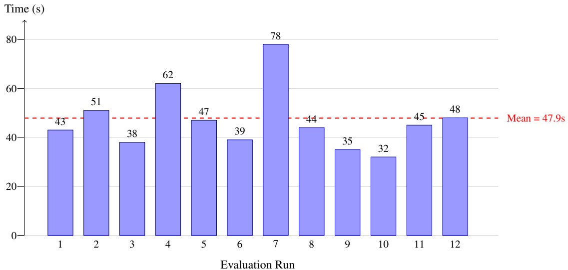
Figure 20: Generation time per evaluation run. The dashed line marks the mean (47.9s). Run 7 is the outlier at 78s due to repeated validation failures.
