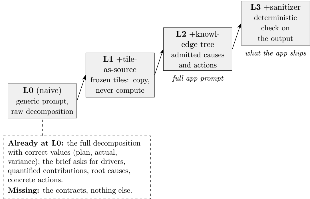
Figure 5.1: The ablation ladder used in the evaluation. Each rung adds one contract on top of the previous level: L2 is the full app prompt, L3 the configuration the app ships. The dashed box lists what the naive baseline already receives; the contracts are the only difference along the ladder.
