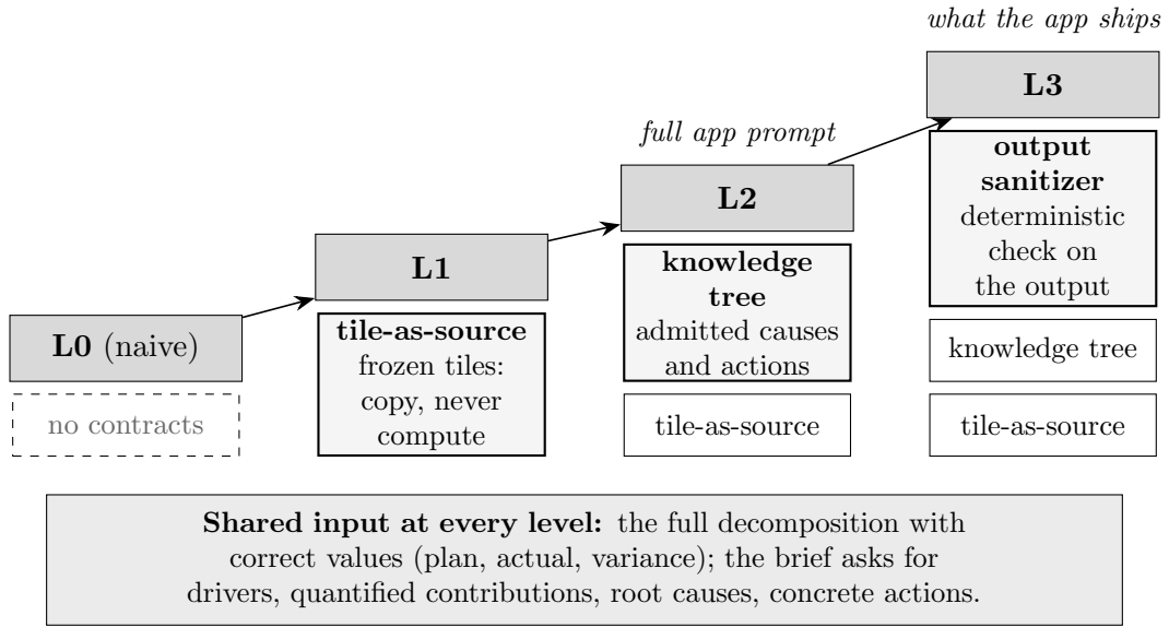
Figure 5.1: The ablation ladder used in the evaluation. All four levels receive the same input (bottom bar); each level stacks one more contract on top of the previous one, and the block with the thick border is the contract that enters at that step. L2 is the full app prompt, L3 the configuration the app ships.
