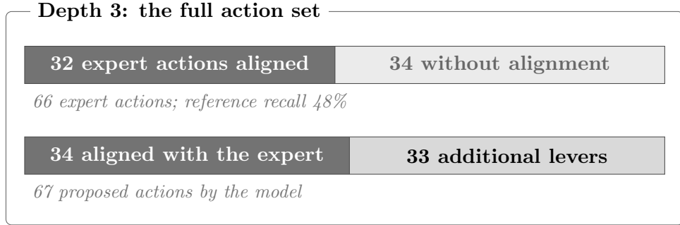
Figure 5.6: Depth 3, the full action set. The upper bar measures reference recall over 66 expert actions; the lower bar describes the 67 actions proposed by the model.
