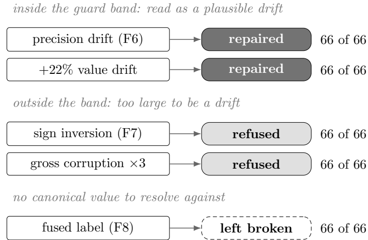
Figure 5.3: The sanitizer stress test: each fault planted on the 66 candidate sites of the shipped narratives. Dark chips are repairs to the canonical value, light chips are refusals that leave the fault visible, and the dashed chip is a fault with no canonical resolution, left untouched. Every outcome is 66 of 66: zero false repairs.
