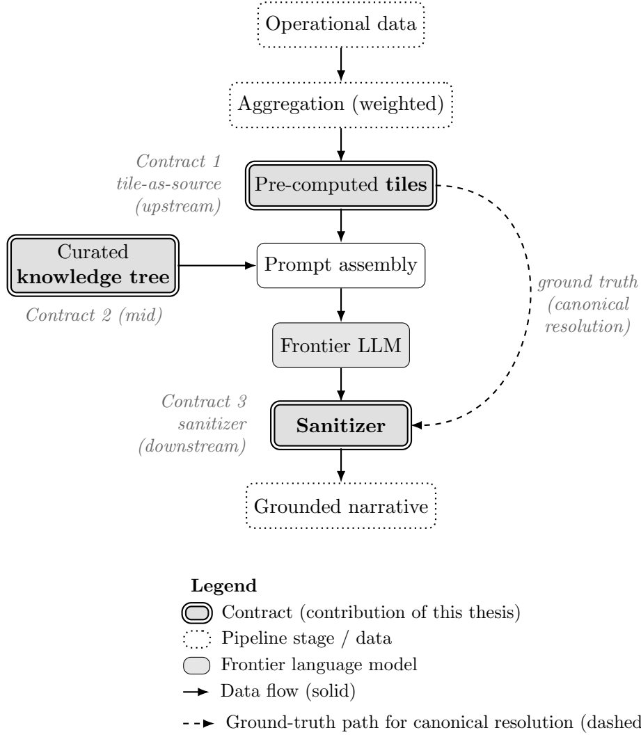
Figure 4.1: The AI-BI pipeline with the three contracts in place, drawn top to bottom.
