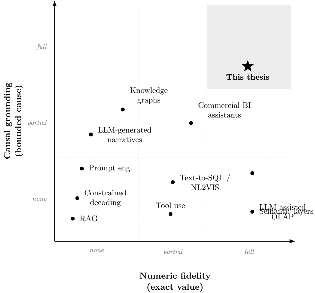
Figure 2.1: The reviewed approaches on the two requirements of operational BI: numeric fidelity (horizontal) and causal grounding (vertical).
