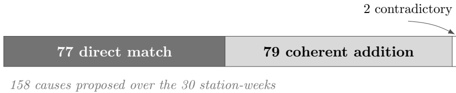
Figure 5.4: The cause set aligned against the expert bridges: of the 158 causes the model proposed, 77 match the expert directly, 79 are additions coherent with the data that the expert did not mention, and 2 contradict the expert’s reading. In-domain adherence is 98.7%.
