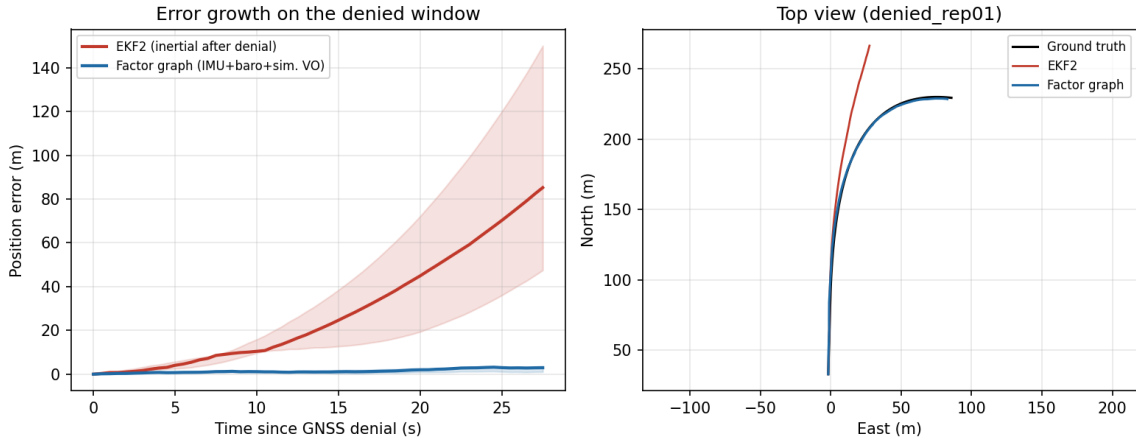
Figure 2: Left: position error after GNSS denial—EKF2 inertial baseline versus a factor-graph smoother on the same logs (median and p05–p95, N=3 ). Right: top view for a representative run.
