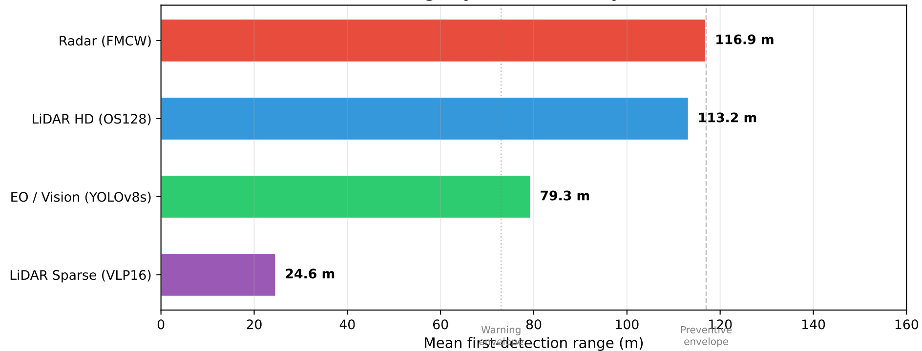
First Detection Range by Sensor Modality — 29 Encounter Runs
