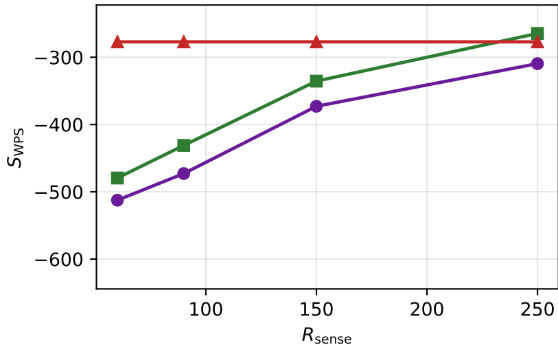
Local sensing ( d = 18 , no share)
