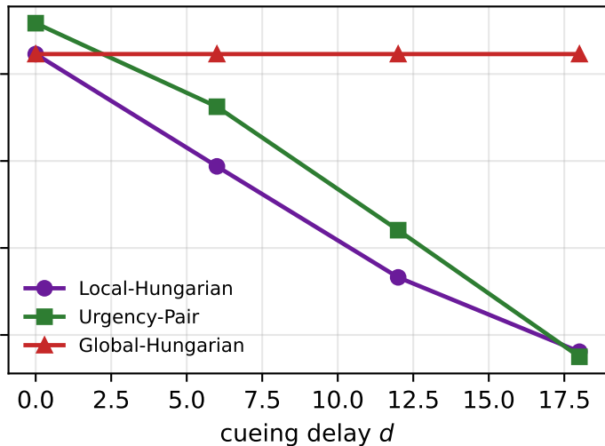
Team cueing ( R = 0 , share)
