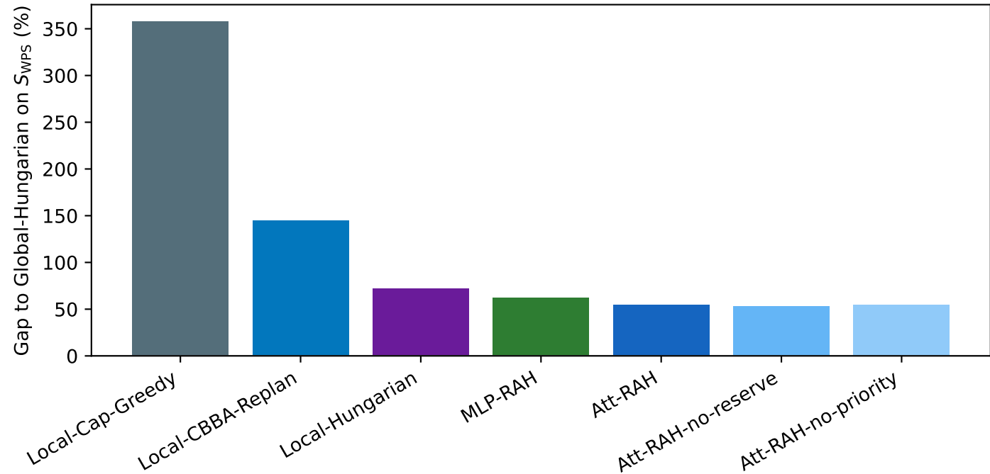
Oracle gap (lower is better)
