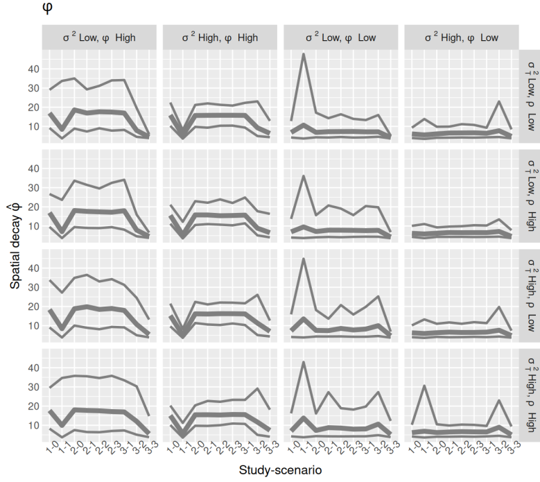
Figure B.10: Point estimates and 95% Credible Intervals (upper and lower bounds) around estimates of the spatial decay parameter \hat{\phi} across studies and scenarios (x-axis). Point estimates were calculated using the 3,000 posterior distribution draws produced by each simulated dataset. Spatial and temporal autocorrelation sub scenarios are represented across columns and rows, respectively.
