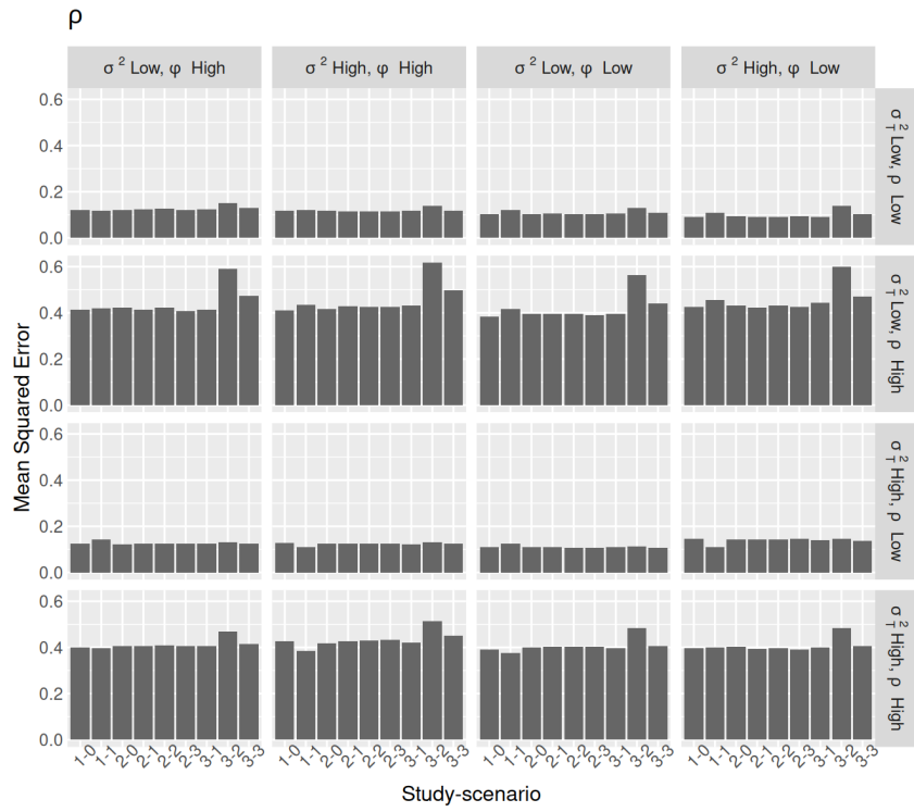
Figure B.24: Mean Squared Error of the temporal autocorrelation \rho estimator across studies, scenarios, and sub scenarios of spatial and temporal autocorrelation (facet labels).
