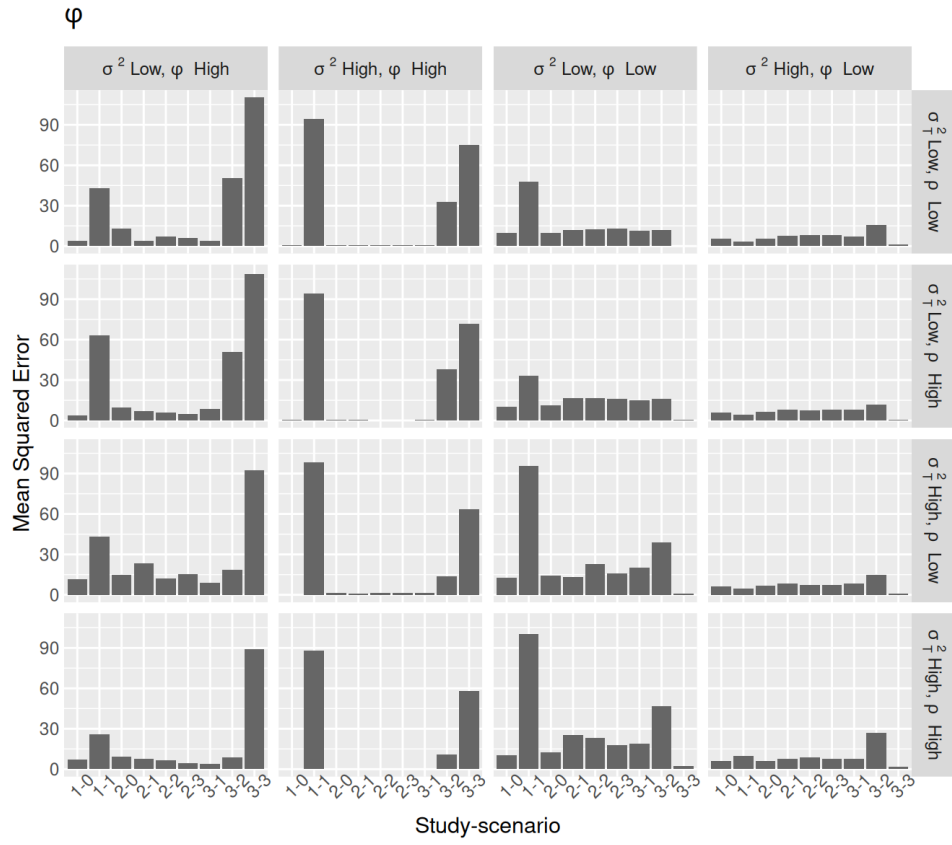
Figure B.22: Mean Squared Error of the spatial decay \phi estimator across studies, scenarios, and sub scenarios of spatial and temporal autocorrelation (facet labels).
