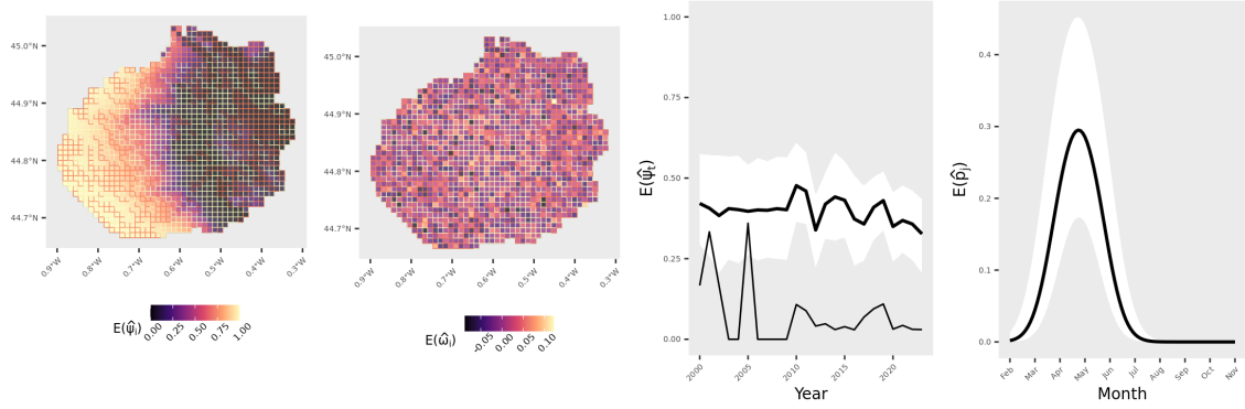
Fig. G.2: Distribution of the marsh fritillary Euphydryas aurinia in Southwest France (buffer of 10 km 2 around Bordeaux). Results for the model with NNGP=15 and weakly informative prior for \phi . Values plotted in the occupancy map (left) were calculated as \mathbb{E}(\hat{\psi}_i) = \frac{1}{T} \sum_{t=1}^T \hat{\psi}_{it} , and refer to in-sample estimates for sites with data (cells with yellow borders) and out-of-sample predictions for missing cells (those with red borders). The spatial random effect \mathbb{E}(\hat{\omega}_i) was also derived from in-sample estimates and out-of-sample predictions from the model. Trend plots show the proportion of occupied sites over the 24 years of data, calculated as \mathbb{E}(\hat{\psi}_t) = \frac{1}{I} \sum_{i=1}^I \hat{\psi}_{it} . The naive occupancy trend (number of sites with detection divided by the total number of sampled sites per year) is depicted by the thinner line. Detection probability over months (secondary periods) was also derived from in-sample predictions. The black line depicts the average detection trend, and the white bands depict the upper and lower bounds of the 95% credible interval. No 1 × 1 km cell was 100% covered by water (the maximum was 93%). Parameter values derived from 1,200 posterior distribution draws.
