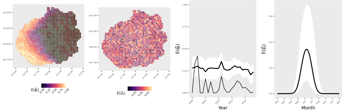
Fig. G.1: Distribution of the false ringlet Coenonympha oedippus in Southwest France (buffer of 10 km 2 around Bordeaux). Results for the model with NNGP=15 and weakly informative prior for \phi . Values plotted in the occupancy map (left) were calculated as \mathbb{E}(\hat{\psi}_i) = \frac{1}{T} \sum_{t=1}^T \hat{\psi}_{it} , and refer to in-sample estimates for sites with data (cells with yellow borders) and out-of-sample predictions for missing cells (those with red borders). The spatial random effect \mathbb{E}(\hat{\omega}_i) was also derived from in-sample estimates and out-of-sample predictions from the model. Trend plots show the proportion of occupied sites over the 24 years of data, calculated as \mathbb{E}(\hat{\psi}_t) = \frac{1}{I} \sum_{i=1}^I \hat{\psi}_{it} . The naive occupancy trend (number of sites with detection divided by the total number of sampled sites per year) is depicted by the thinner line. Detection probability over months (secondary periods) was also derived from in-sample predictions. The black line depicts the average detection trend, and the white bands depict the upper and lower bounds of the 95% credible interval. No 1 × 1 km cell was 100% covered by water (the maximum was 93%). Parameter values derived from 1,200 posterior distribution draws.
