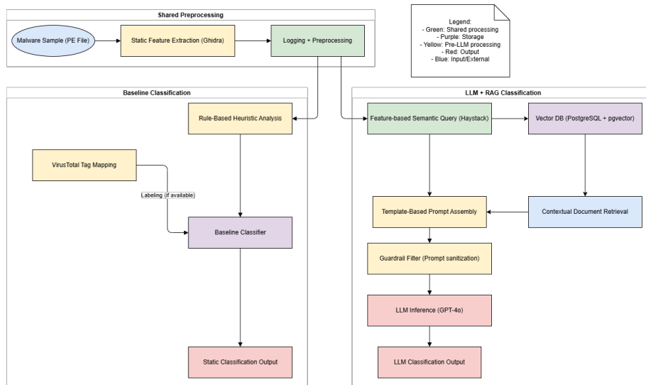
FIGURE 3.1: System architecture showing baseline and LLM+RAG pipelines
